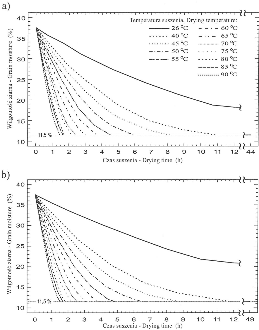
Rys. 4. Krzywe suszenia ziarna pszenicy odmian Roma (a) i Igna (b) Fig. 4. Drying curves of wheat grain for cultivars Roma (a) and Igna (b)
