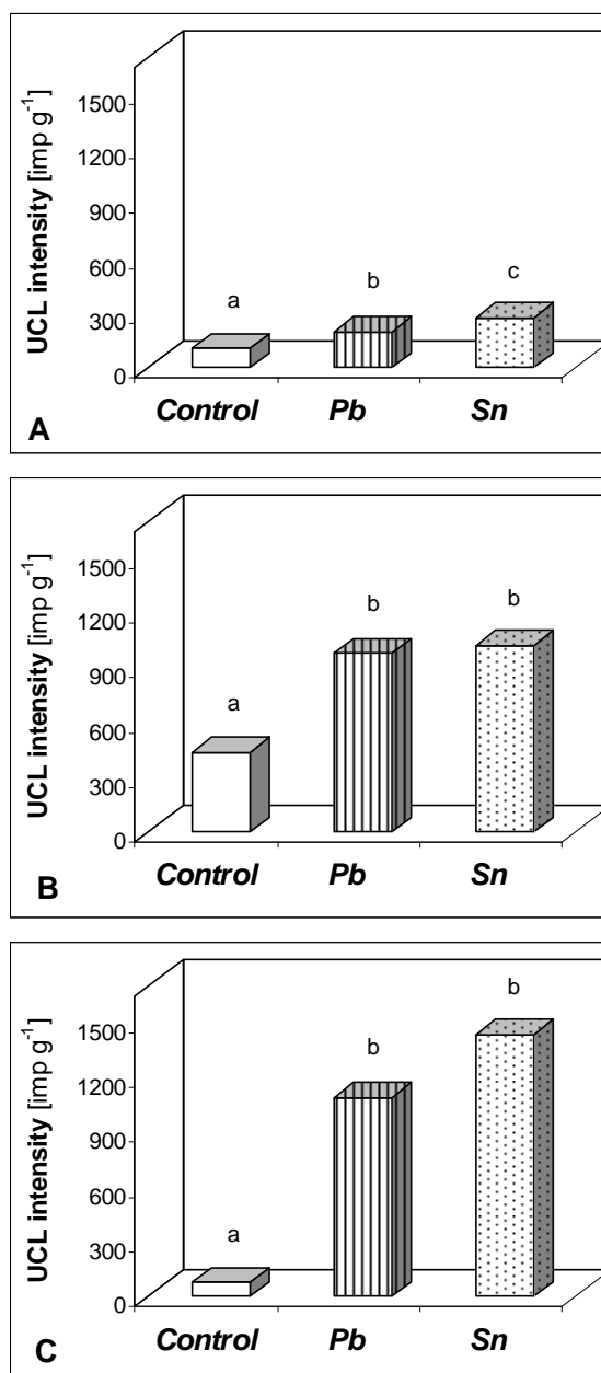
Fig. 3. Values of UCL intensity per 1 g of dry mass of cucumber leaf disc after 20 h treatment by 2 \mu\text{mol dm}^{-3} of (\text{C}_6\text{H}_5)_3\text{PbCl} or (\text{C}_6\text{H}_5)_3\text{SnCl} in darkness at temperature of 21^\circ\text{C} (A, experiment 1), after 2 h at 3^\circ\text{C} at PPF 1200 \mu\text{mol m}^{-2} \text{s}^{-1} (B, experiment 2), and after 20 h of recovery (C, experiment 3)
