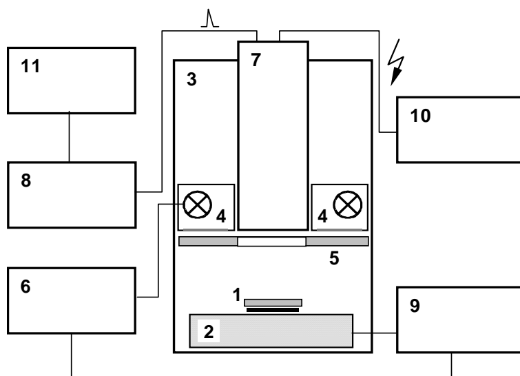
Fig. 2. Special luminometer for recording chlorophyll delayed luminescence decay 1 – investigated leaf disc covered by a glass plate; 2 – drawer with table for investigated sample; 3 – light-proof measuring camera; 4 – illuminator; 5 – mechanical diaphragm; 6 – power supply of the illuminator; 7 – photomultiplier Zeiss S52FC20 (photocathode S20) with preamplifier; 8 – counter; 9 – power supply of thermoelectric battery; 10 – high voltage power supply; 11 – printer
