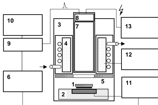
Fig. 1. Ultraweak biochemiluminescence measurement set
