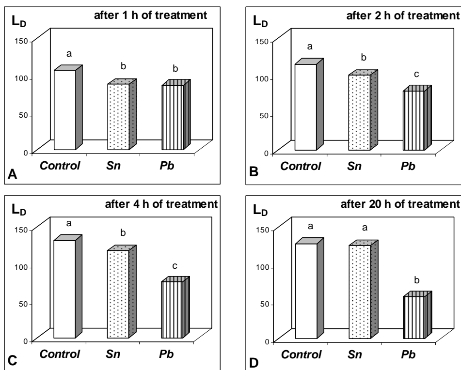
Fig. 4. Values of L_D , rate of delayed luminescence decay of Scenedesmus quadricauda , measured after 1 h (A), 2 h (B), 4 h (C) and 20 h (D) of treatment by 0.5 \mu\text{mol dm}^{-3} of (\text{C}_6\text{H}_5)_3\text{PbCl} or (\text{C}_6\text{H}_5)_3\text{SnCl}
